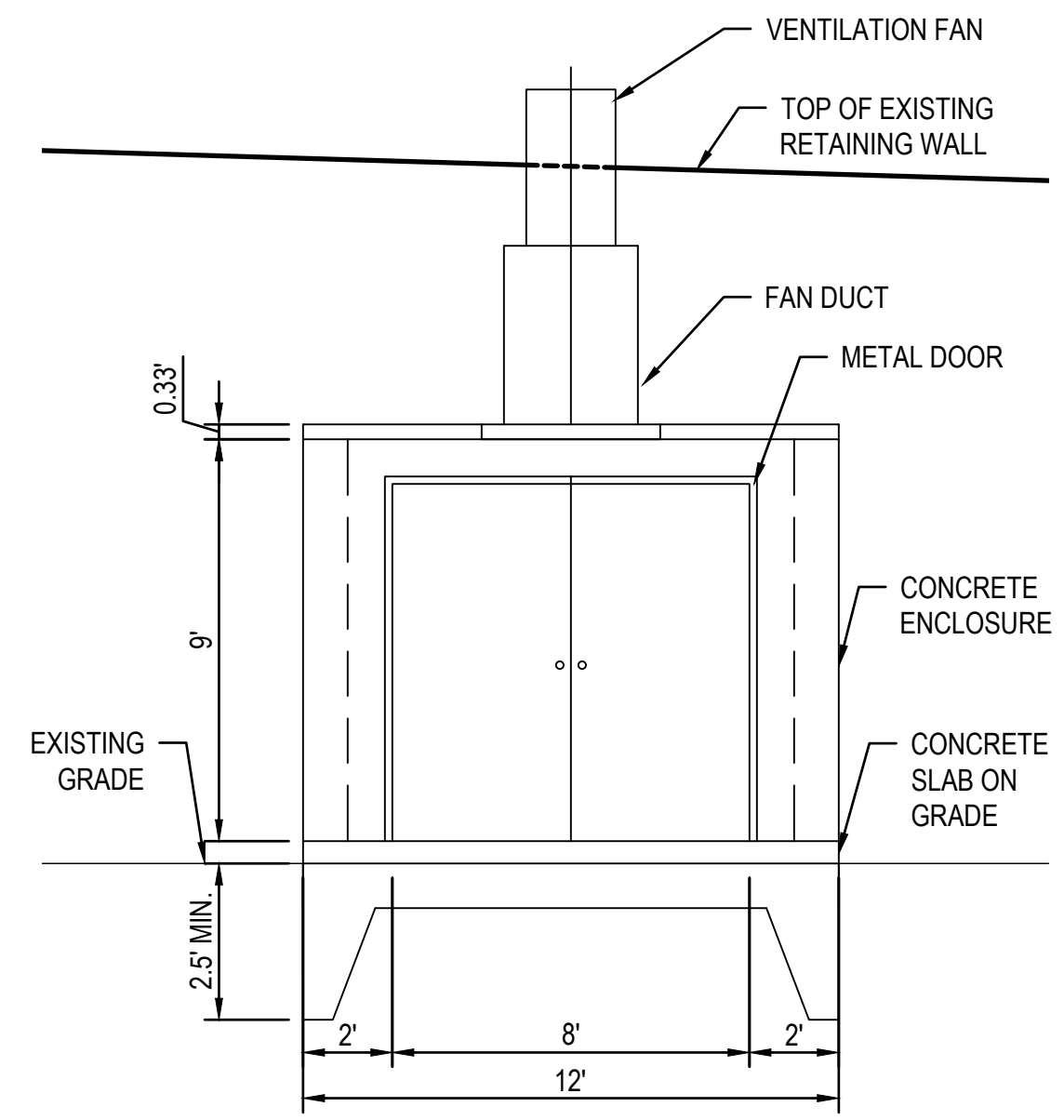
2 NORTH ESCAPE TUNNEL VESTIBULE PLAN & PROFILE NTS
